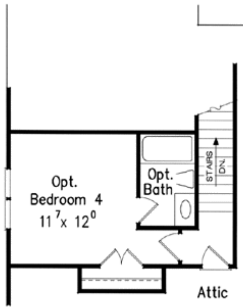
OPT. SECOND FLOOR
